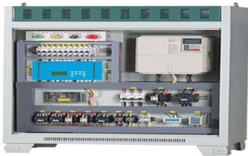
CONTROL PANEL WITH V3F DRIVE
